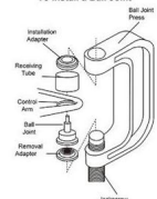
To Install a Ball Joint
